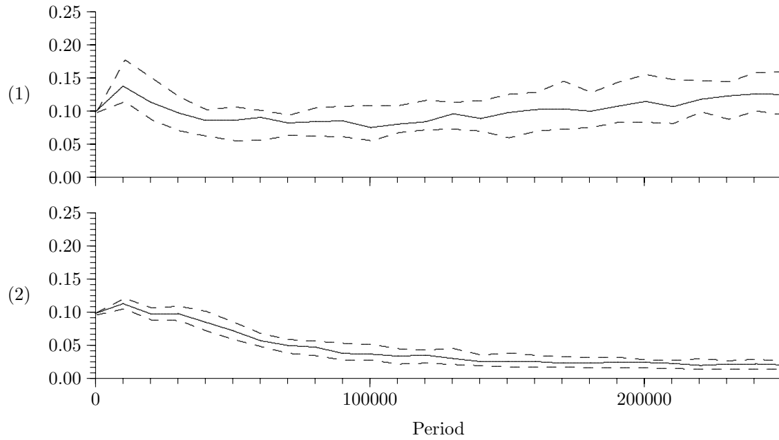
Figure 5: Technical Trading Bits (1) Fast Learning, (2) Slow Learning. Median and 25/75 Quantiles: 25 runs
