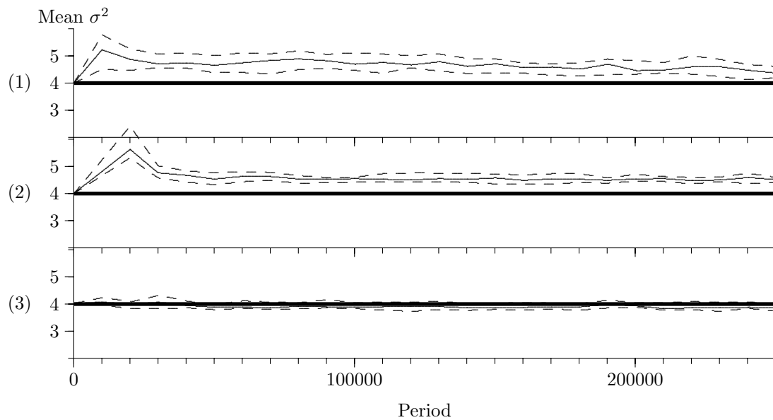
Figure 9: Mean Variance Estimate \sigma^2
