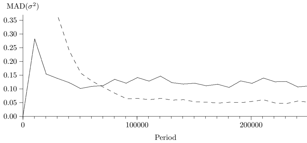
Figure 10: Mean Absolute Deviation for Variance Estimate \sigma^2 Fast Learning: solid, Slow Learning: dashes
