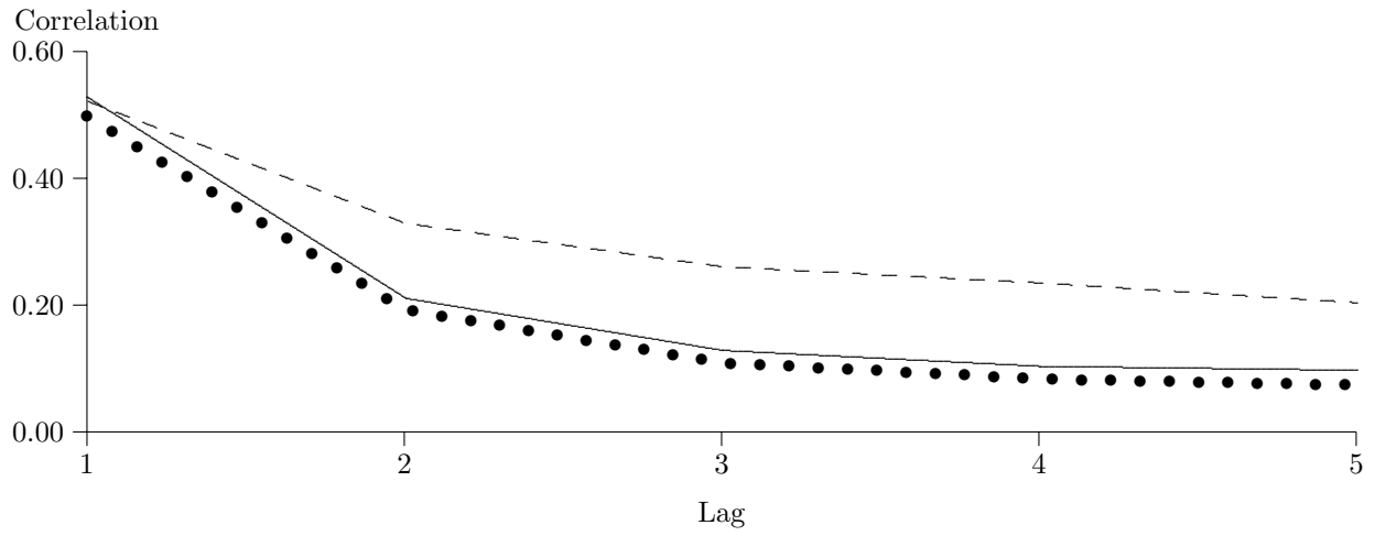
Figure 2: Volume Autocorrelations
