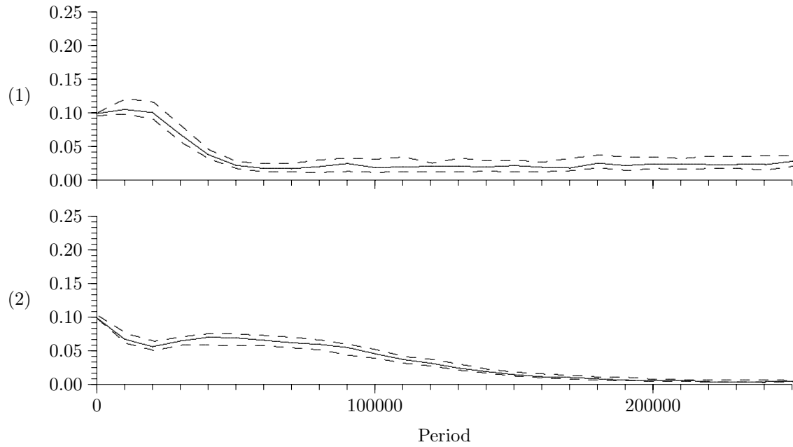
Figure 4: Average Bits Set
