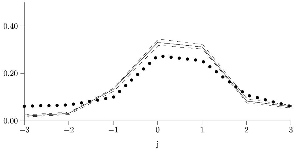
Figure 3: Crosscorrelations: Squared Returns and Trading Volume
